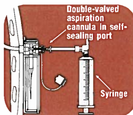
Double-valved aspiration cannula allows immediate manual air evacuation.
